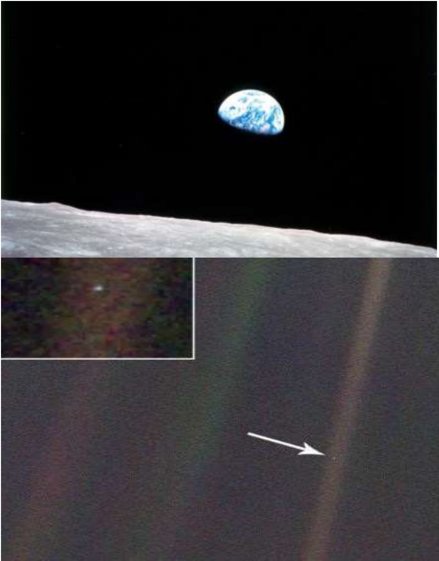
Above: Earth rising above Moon. Below: Pale Blue Dot Earth taken by Voyager 1 spacecraft, from 4 billion miles away.
